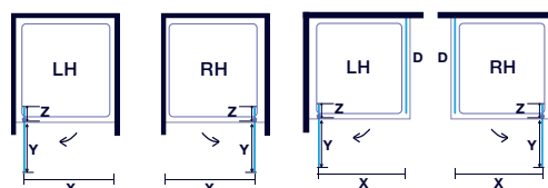
Pivot Door in Recess
