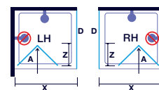
Bifold Door with Side Panel
