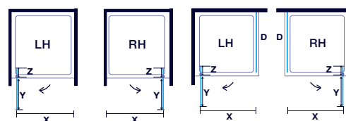
Pivot Door in Recess
