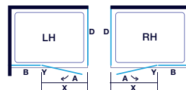
Hinge and Inline Door with Side Panel
