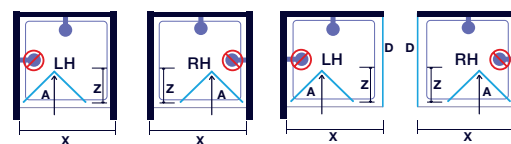
Bifold Door in Recess
