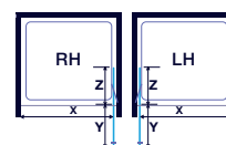
Infold Door in Recess
